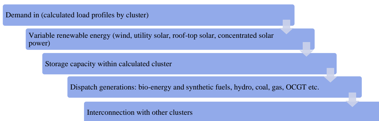
Figure 36: Dispatch order within one cluster
